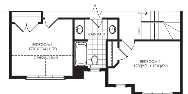
PARTIAL OPT. 4 BEDROOM SECOND FLOOR EL. B
