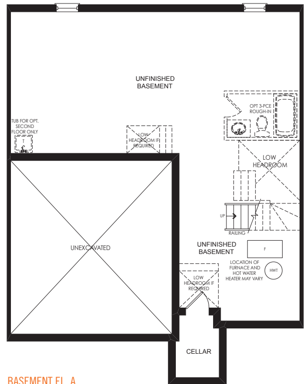
BASEMENT EL. A
