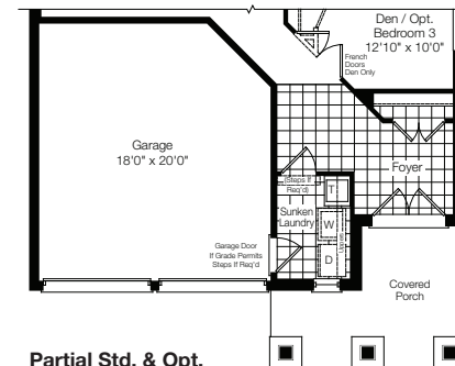
Partial Std. & Opt. Ground Floor Elev. 'B'
