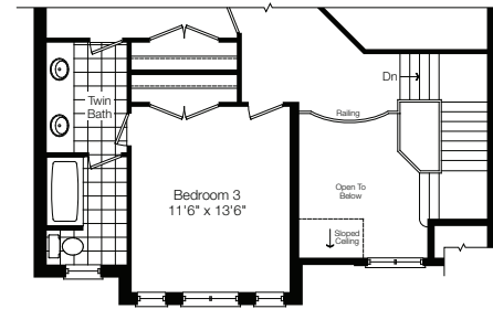
Partial Ground Floor Elev. 'B'
