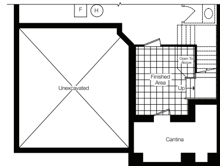
Partial Basement Floor Elev. 'B'
