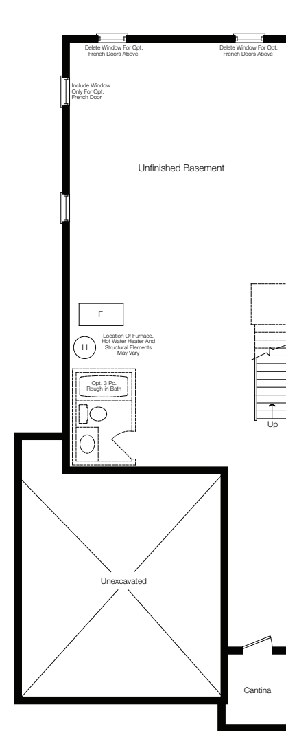
Basement Floor Elev. 'A' & 'B'
