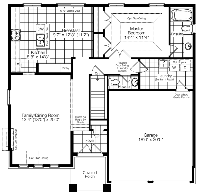
Ground Floor Elev. 'B'
