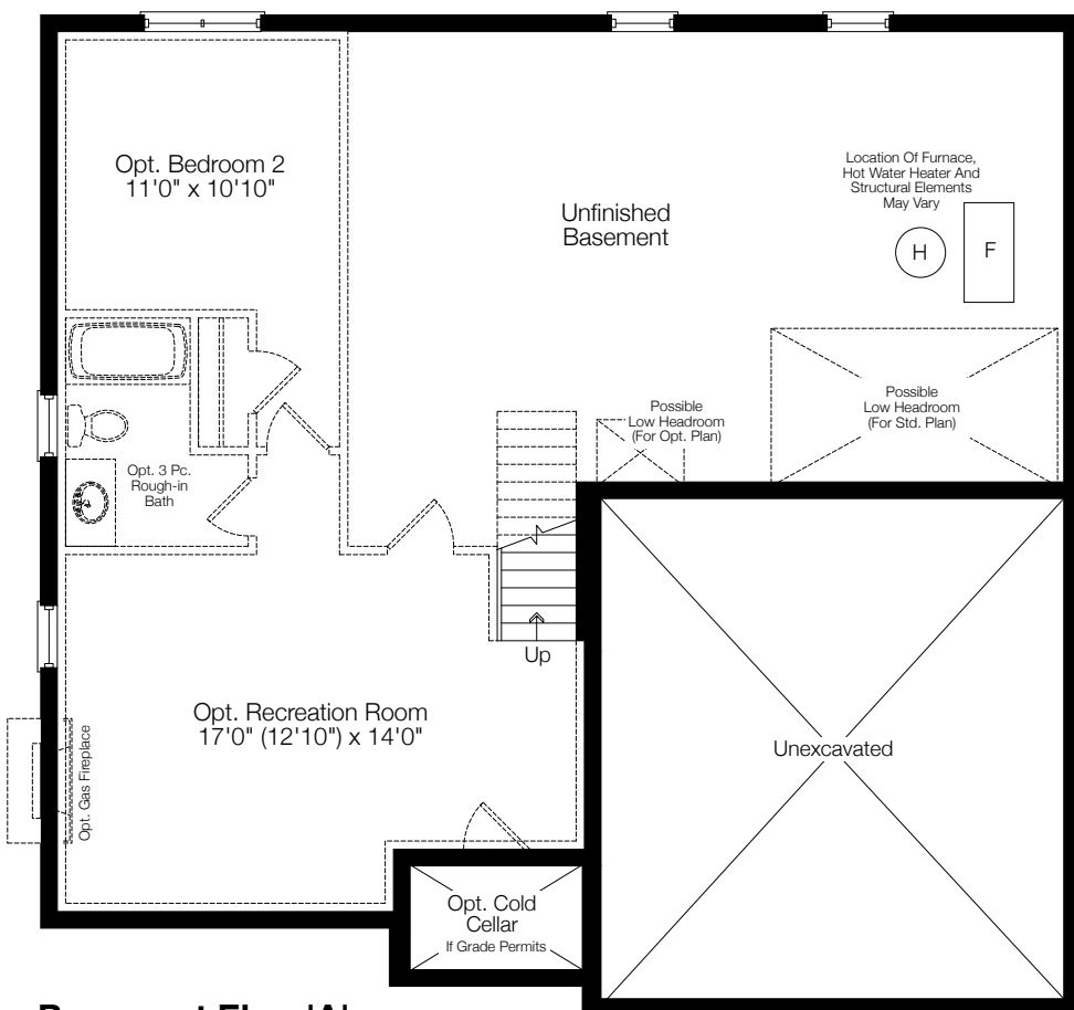
Basement Elev. 'A'
