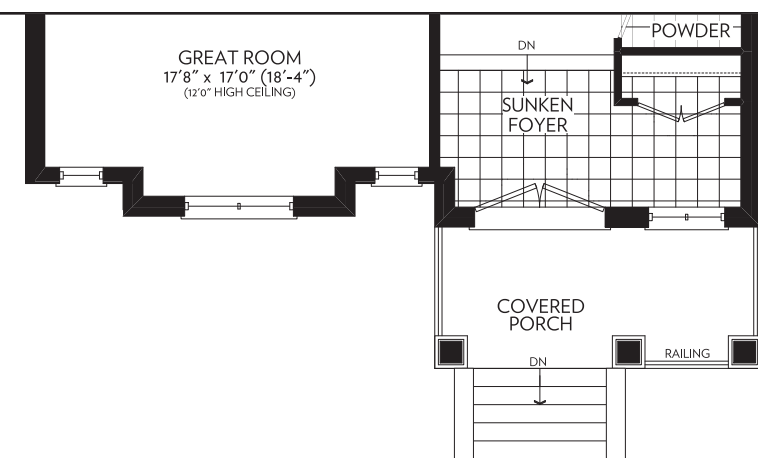
GROUND FLOOR PARTIAL ELEVATION B
