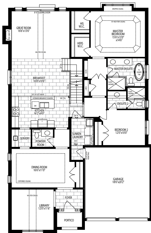
GROUND FLOOR W/OPT. LOFT EL A
