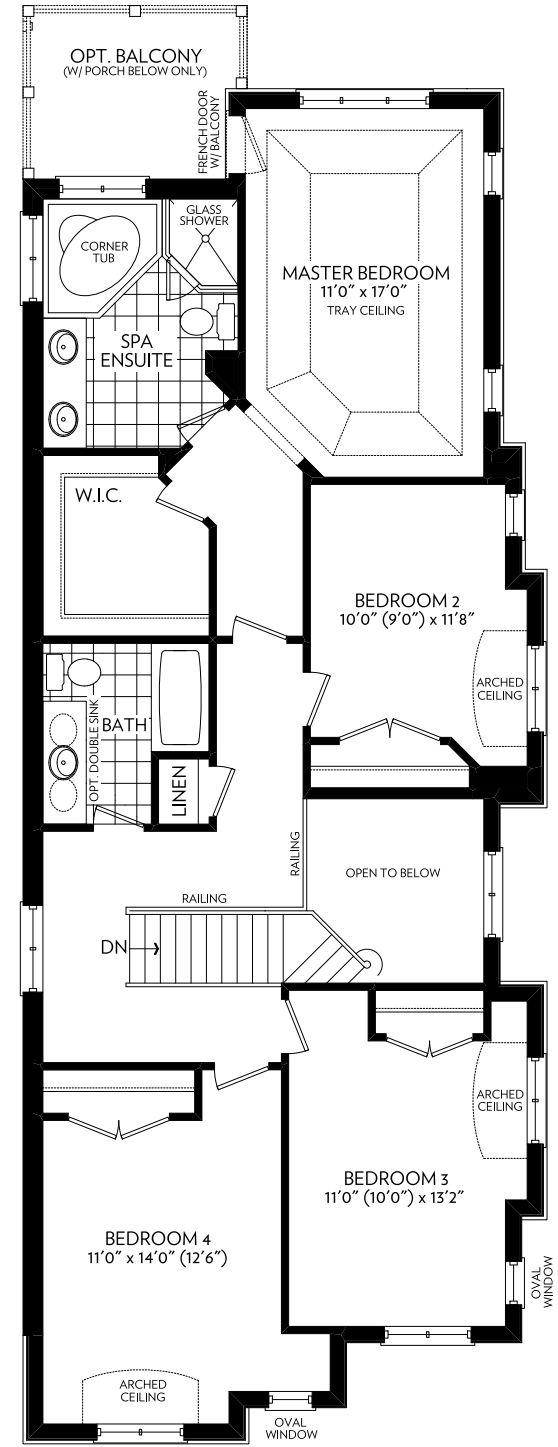
SECOND FLOOR ELEVATION B
