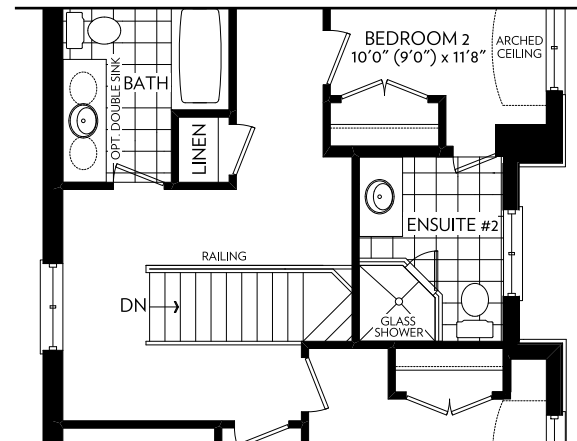
OPT. 3 BATHROOM SECOND FLOOR PARTIAL ELEVATION B
