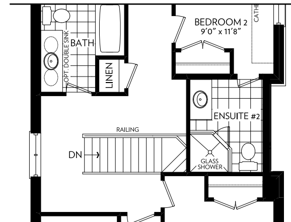
OPT. 3 BATHROOM SECOND FLOOR PARTIAL ELEVATION A
