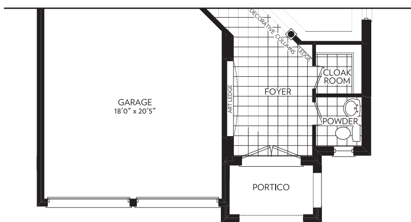
GROUND FLOOR PARTIAL ELEVATION B
