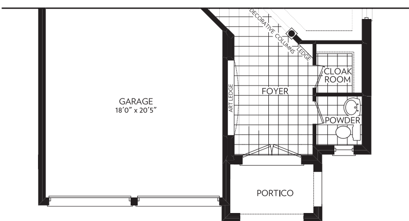
OPT. GROUND FLOOR WITH DEN PARTIAL ELEVATION B
