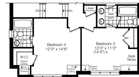
Partial Second Floor Elev. 'B'
