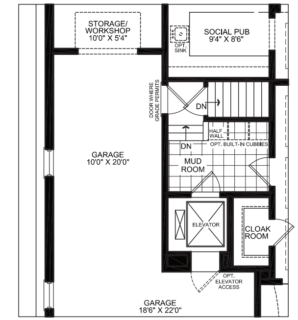
PARTIAL GROUND FLOOR OPTIONAL ELEVATOR IN LIEU OF W.I.C.
