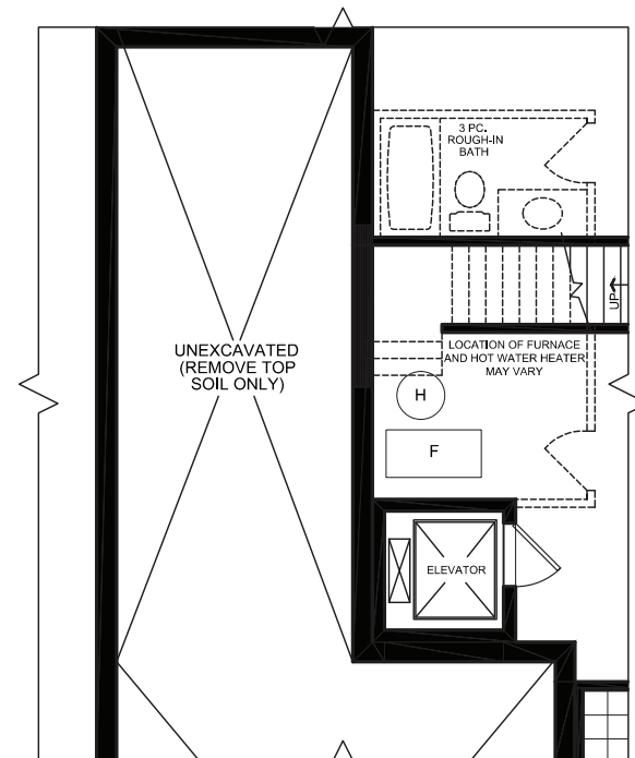
PARTIAL BASEMENT PLAN W/ OPT. ELEVATOR
