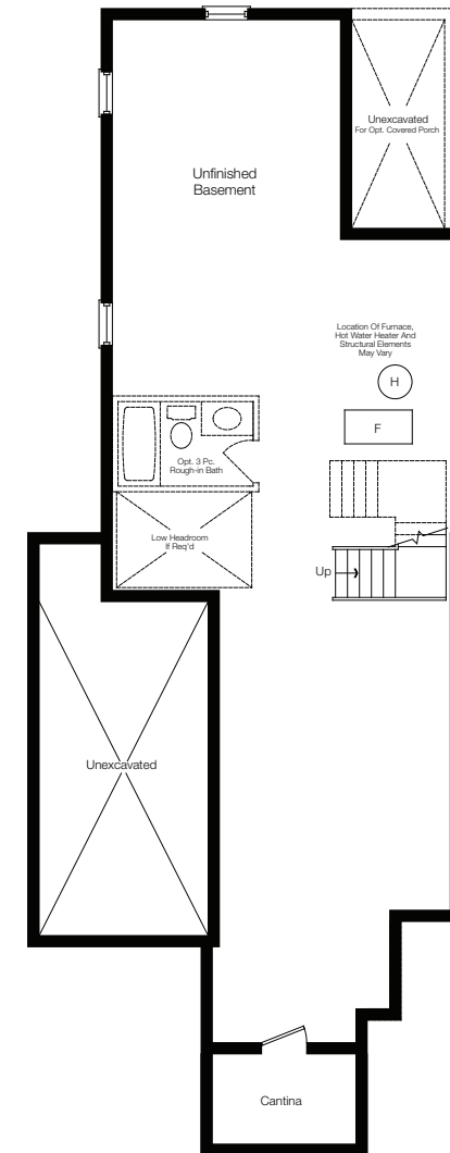
Basement Floor Elev. 'A'
