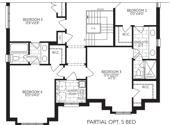
OPT. 5 BED SECOND FLOOR PLAN, EL. 'A'
