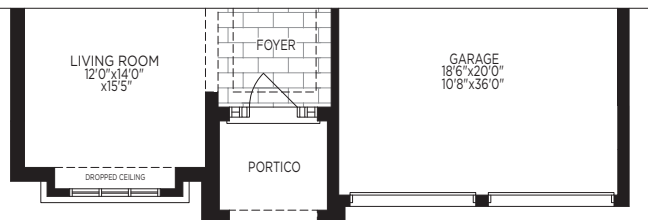
PARTIAL GROUND FLOOR PLAN, EL. 'B'
