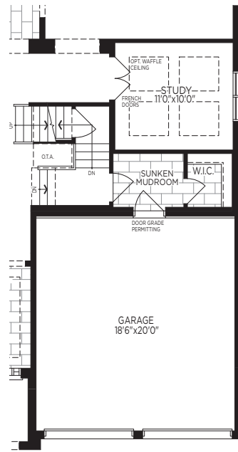
PARTIAL OPT. GROUND FLOOR PLAN W/ STUDY
