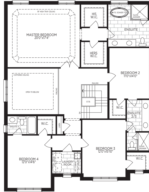
SECOND FLOOR PLAN, EL. 'A'
