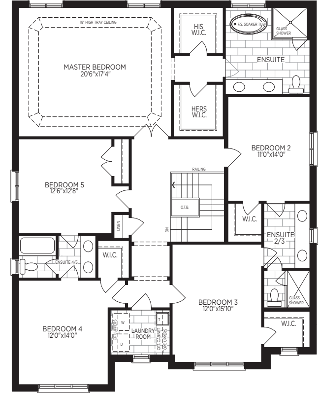
OPT. 5 BED SECOND FLOOR PLAN, EL. 'A'
