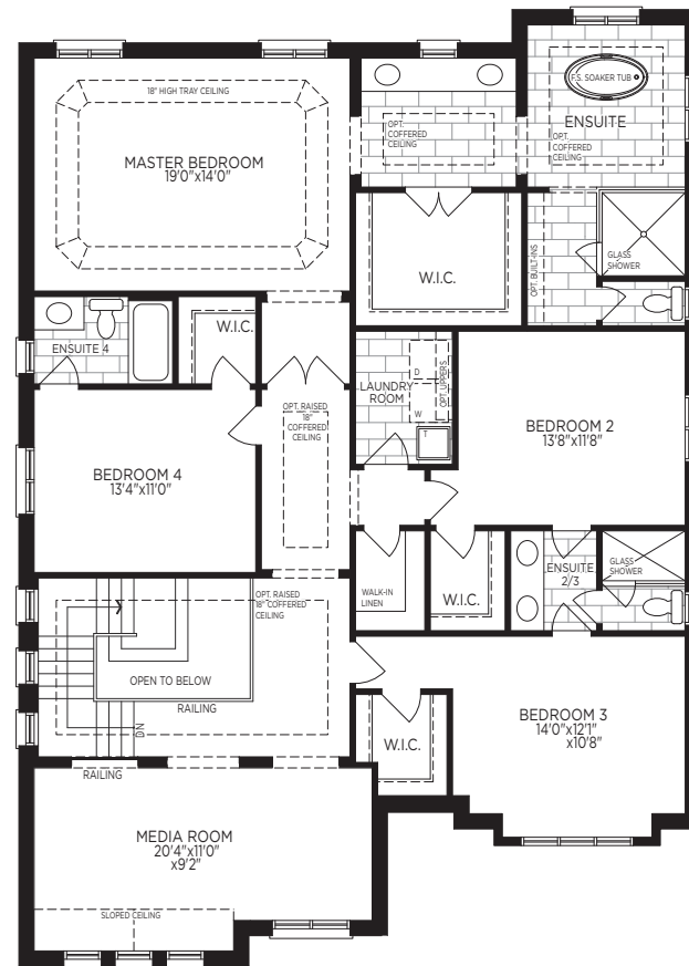
SECOND FLOOR PLAN, EL. 'A'
