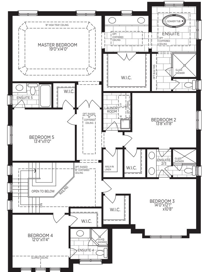
OPT. SECOND FLOOR PLAN, EL. 'A'
