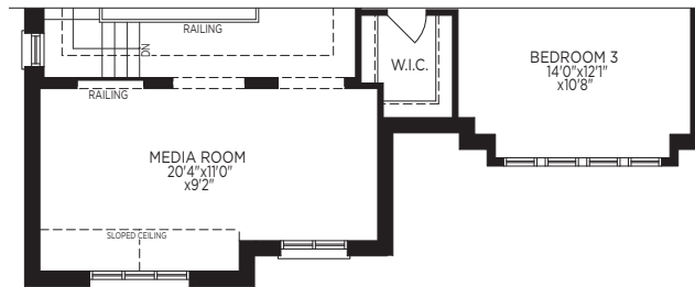
PARTIAL SECOND FLOOR PLAN, EL. 'B'
