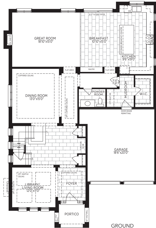
GROUND FLOOR PLAN, EL. 'A'
