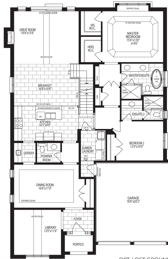
OPT. LOFT GROUND FLOOR PLAN, EL. 'A'
