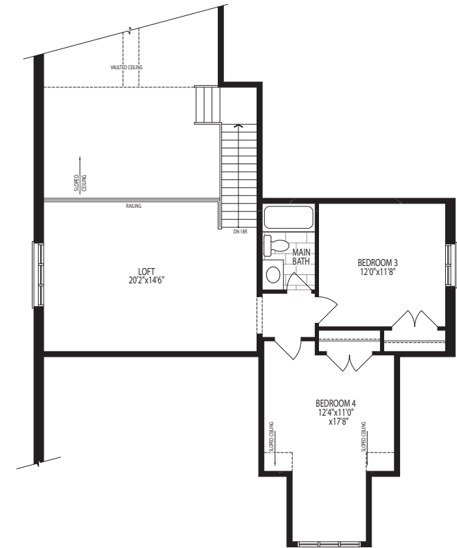
OPT. LOFT FLOOR PLAN, EL. 'A' & 'B'
