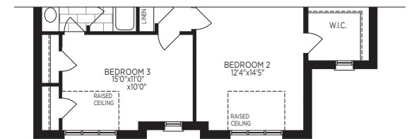
PARTIAL SECOND FLOOR PLAN, EL. 'B'
