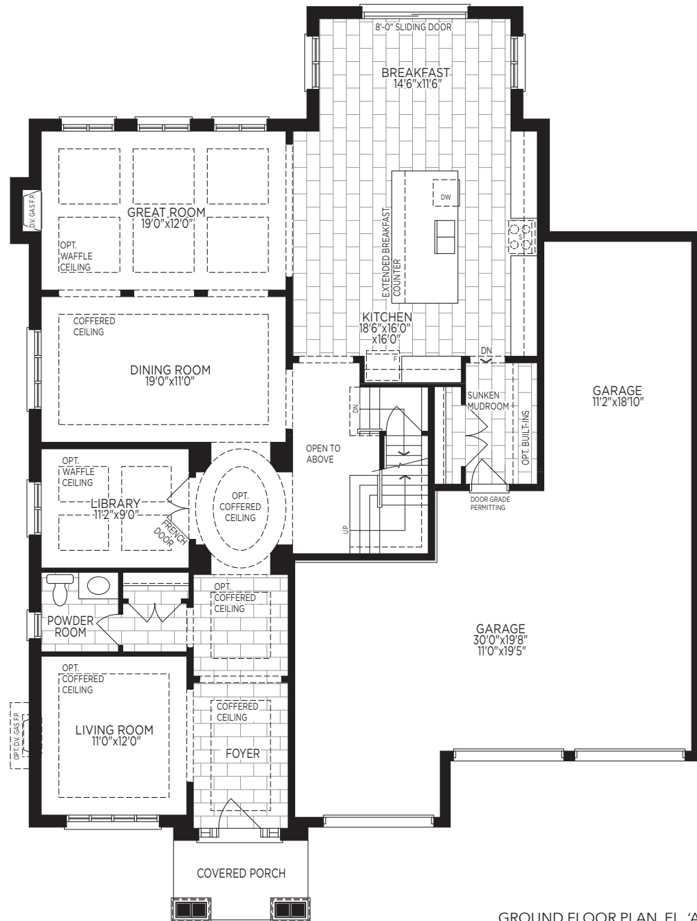
GROUND FLOOR PLAN, EL. 'A'
