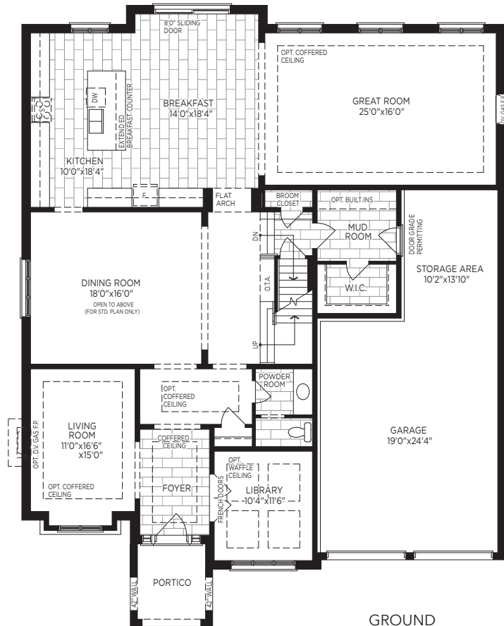
GROUND FLOOR PLAN, EL. 'A'
