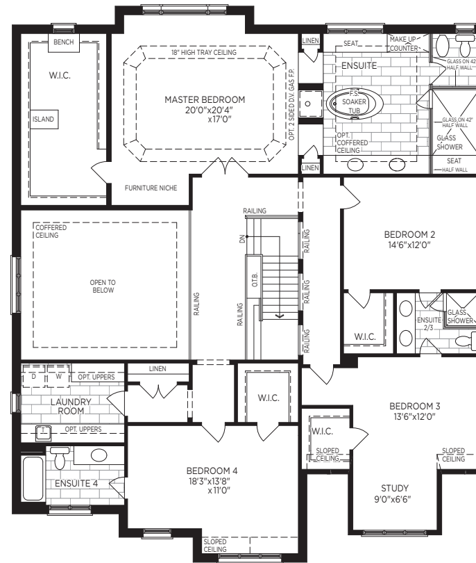
SECOND FLOOR PLAN, EL. 'A'
