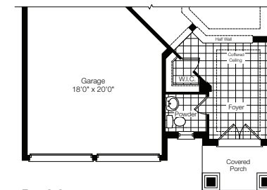
Partial Ground Floor Elev. 'B'
