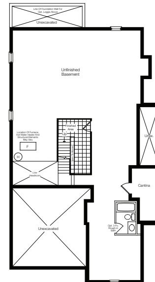
Basement Floor Elev. 'B'
