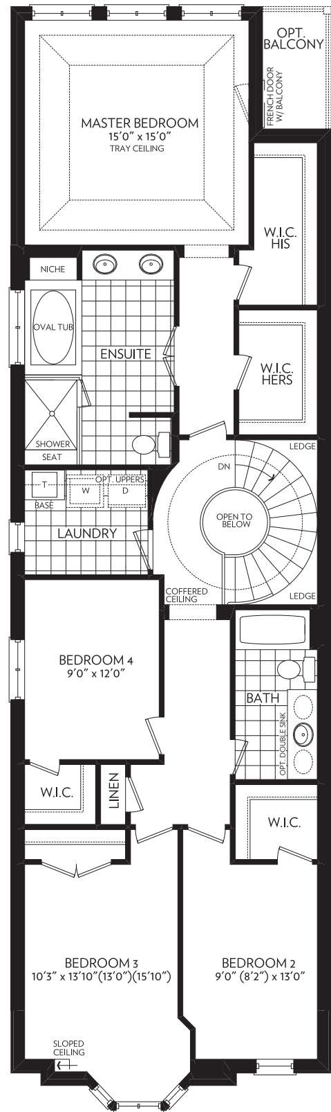
SECOND FLOOR ELEVATION A
