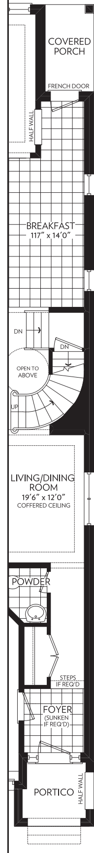
GROUND FLOOR END CONDITION PARTIAL ELEVATION A
