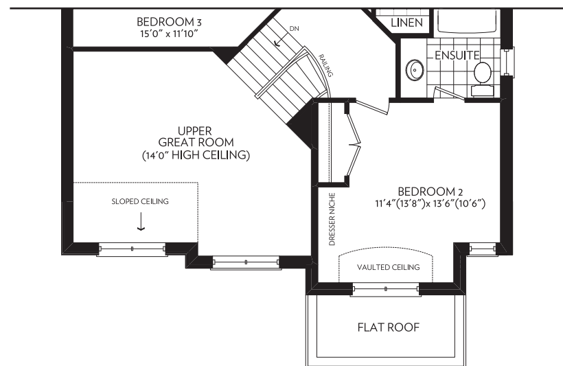
SECOND FLOOR PARTIAL ELEVATION B
