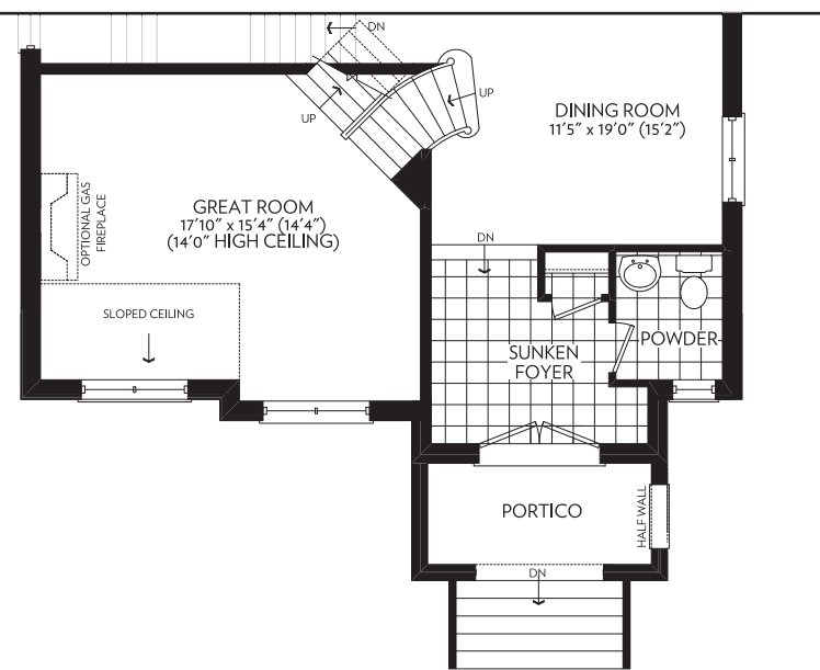
GROUND FLOOR PARTIAL ELEVATION B
