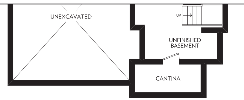
BASEMENT PARTIAL ELEVATION B
