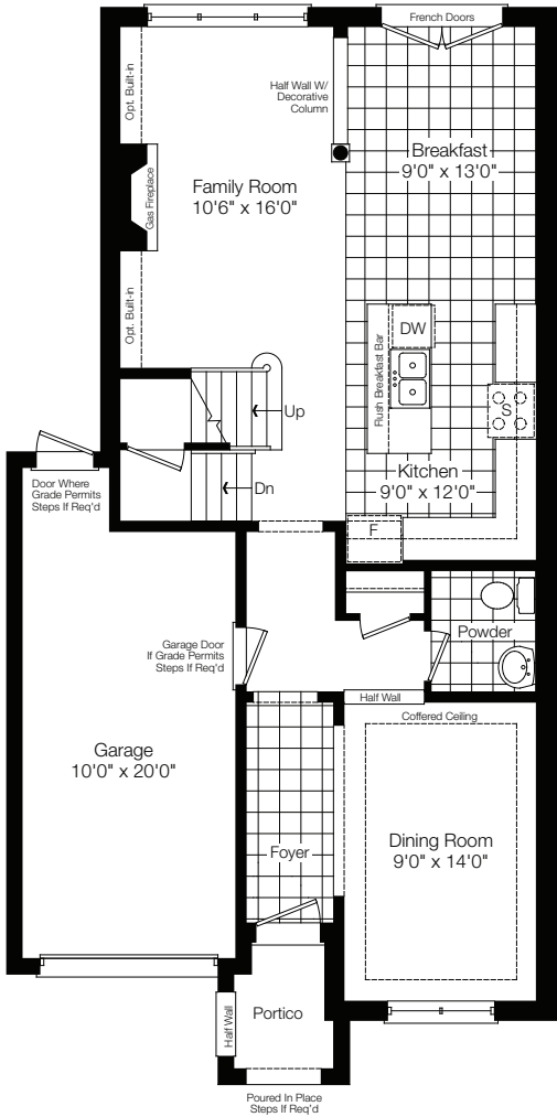
Ground Floor Elev. 'A'
