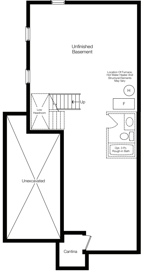
Basement Floor Elev. 'A'
