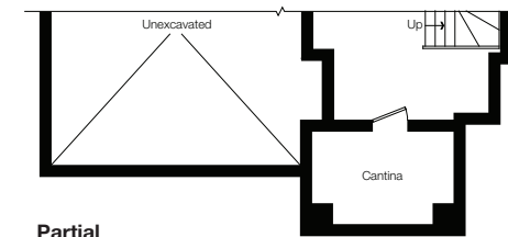
Partial Basement Floor Elev. 'B'
