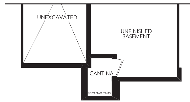
BASEMENT PARTIAL ELEVATION B
