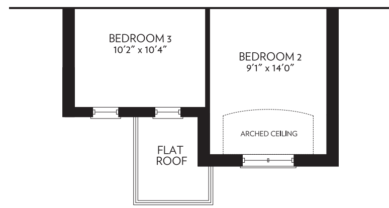
SECOND FLOOR PARTIAL ELEVATION B
