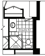
Second Floor Elev. 'A' & 'B' Opt. 3 Bath Plan
