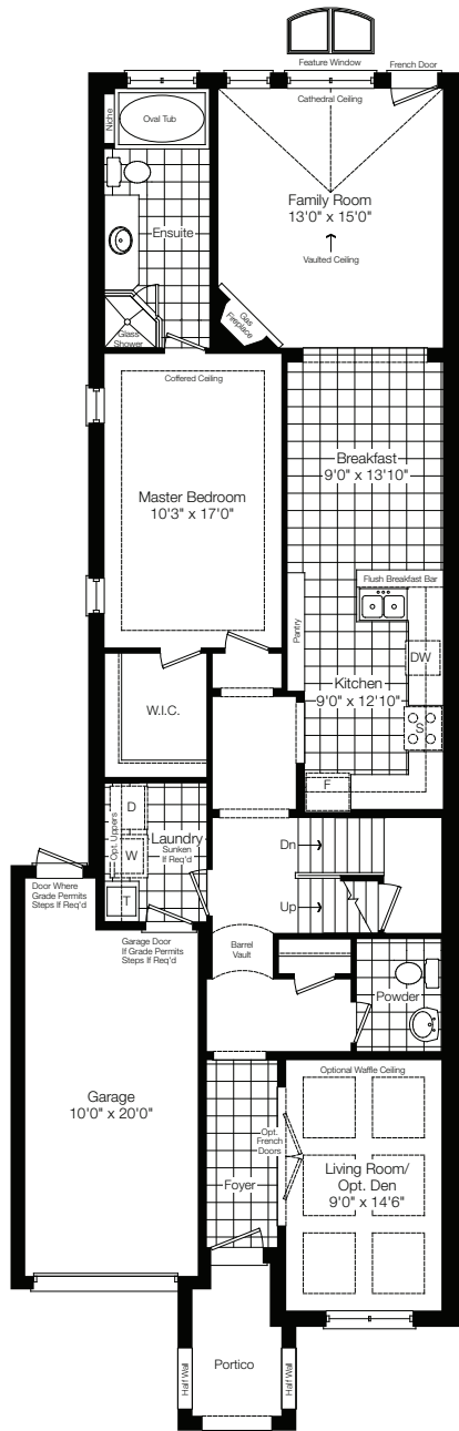
Ground Floor Elev. 'A'
