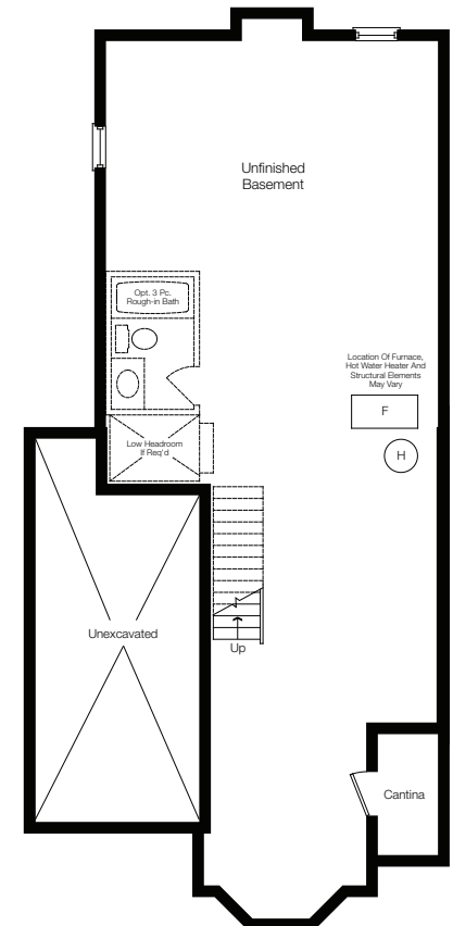
Basement Floor Elev. 'A'
