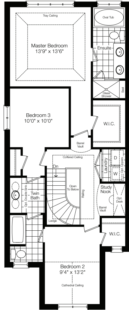
Second Floor Elev. 'A'
