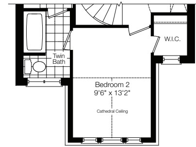
Partial Second Floor Elev. 'B'
