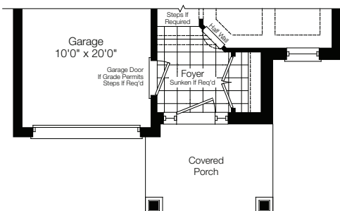
Partial Ground Floor Elev. 'B'
