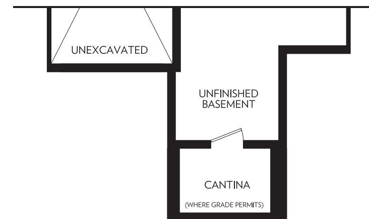
BASEMENT PARTIAL ELEVATION B
