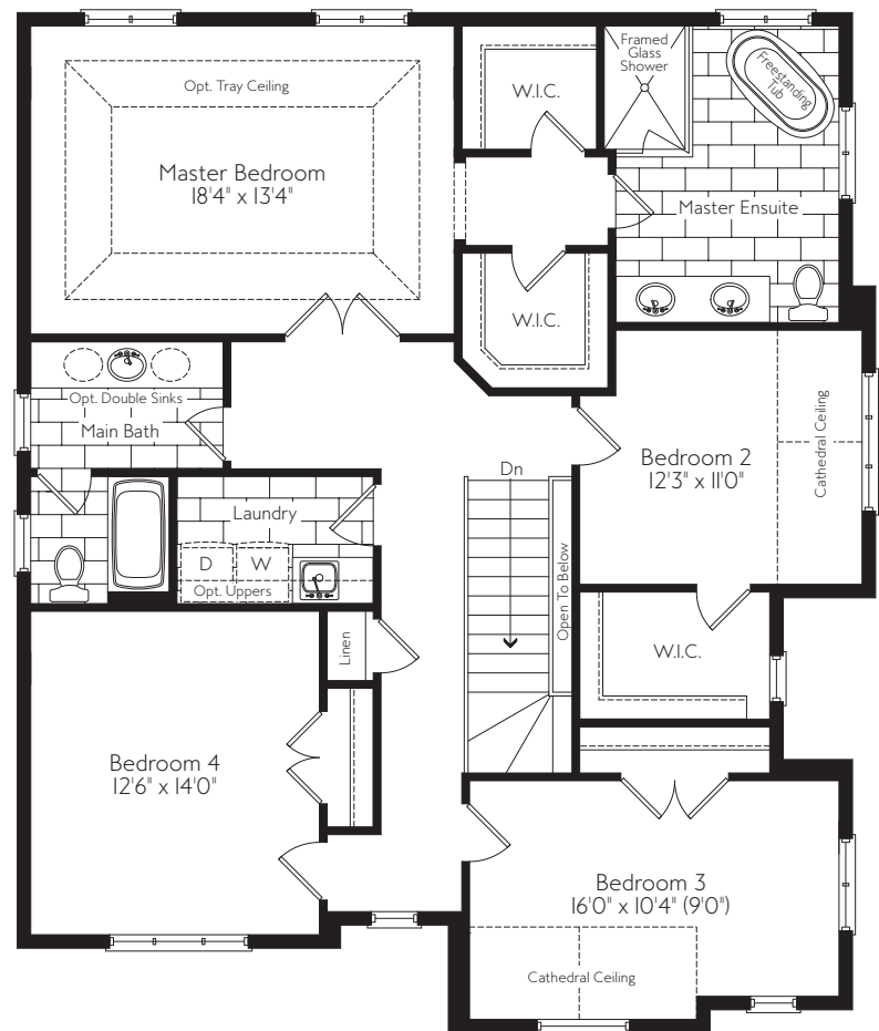
SECOND FLOOR ELEVATION A
