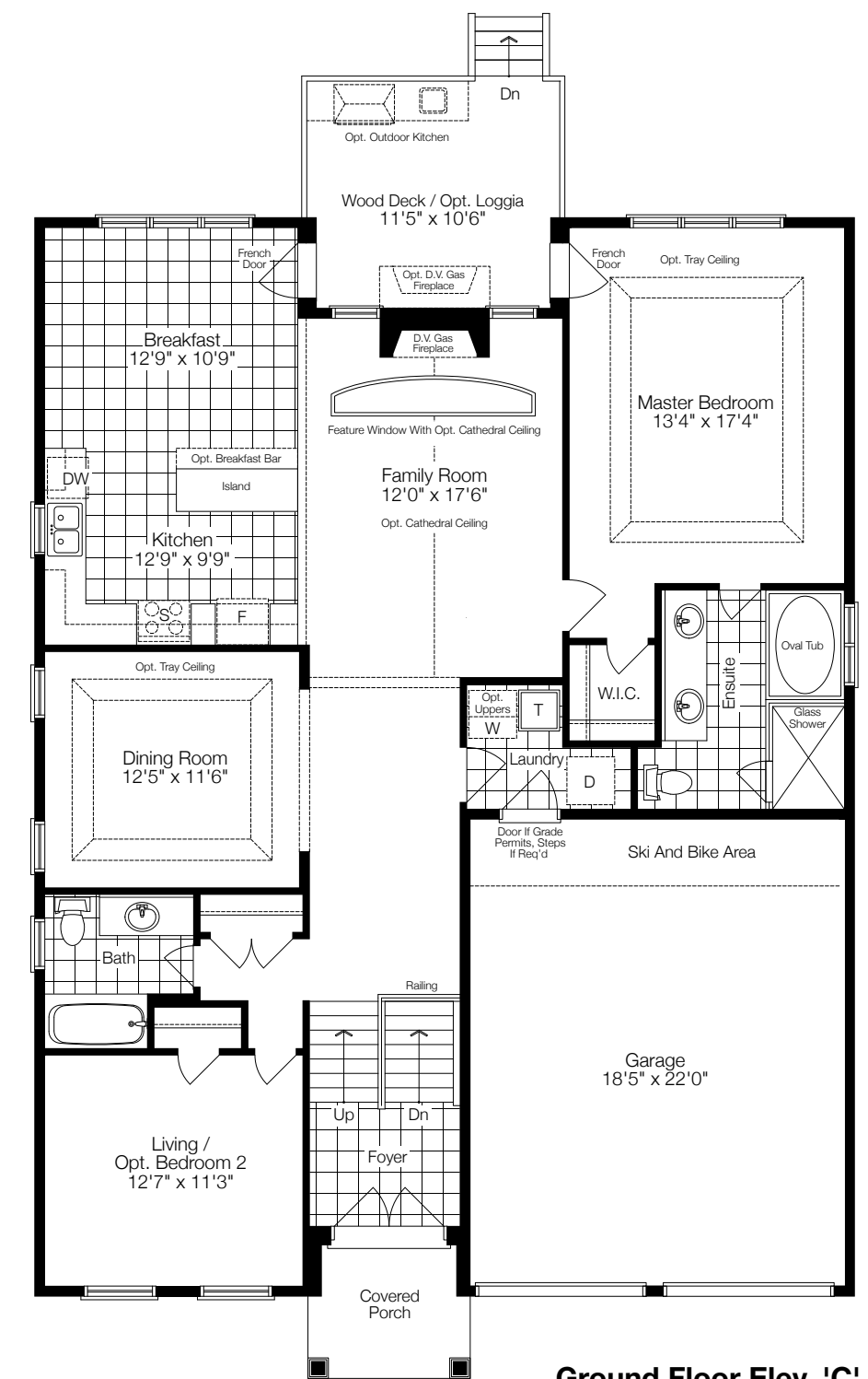
Ground Floor Elev. 'C'
