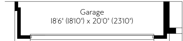
PARTIAL GROUND FLOOR ELEVATION B WITH 16FT. GARAGE DOOR
