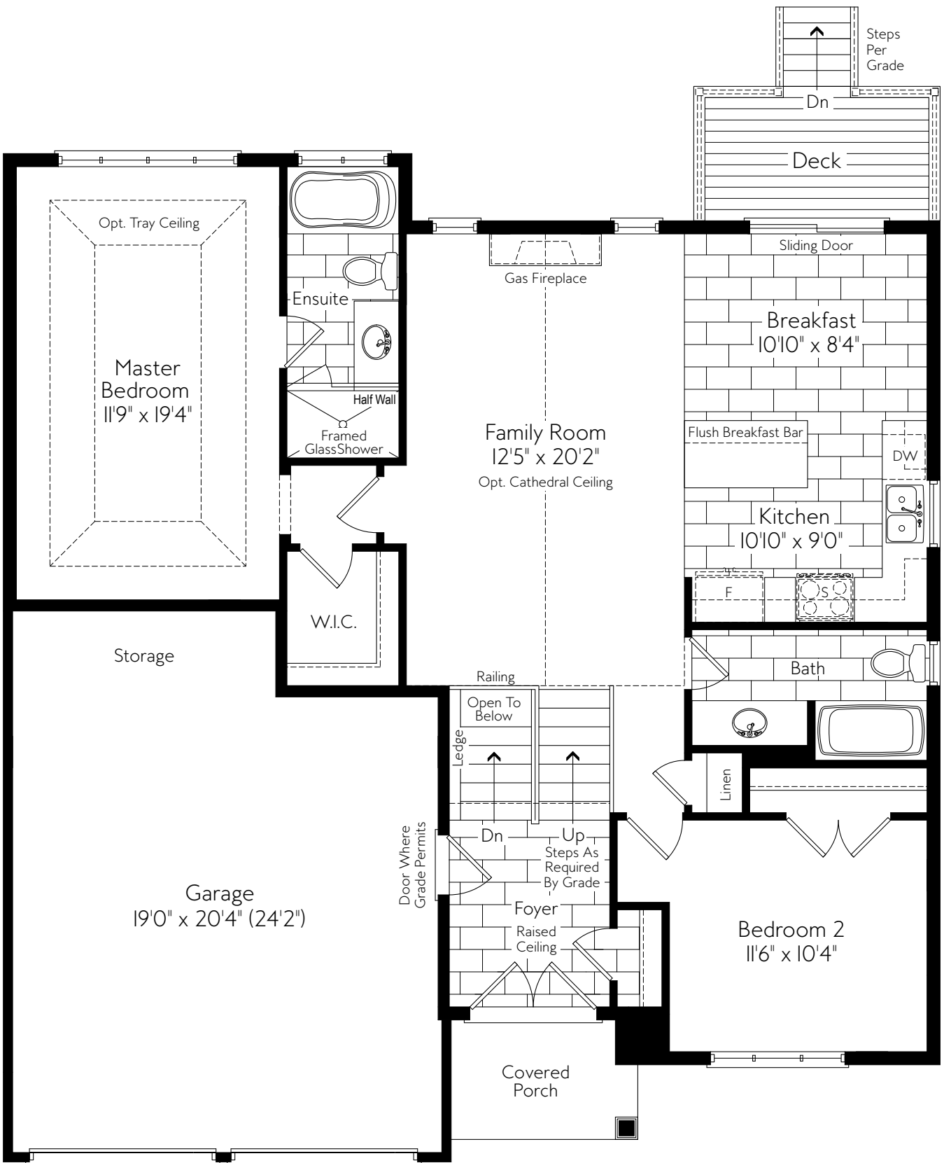
GROUND FLOOR ELEVATION A
