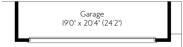
PARTIAL GROUND FLOOR ELEVATION A WITH 16FT. GARAGE DOOR
