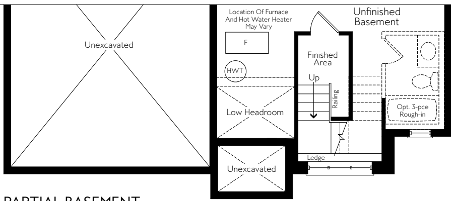
PARTIAL BASEMENT ELEVATION B
