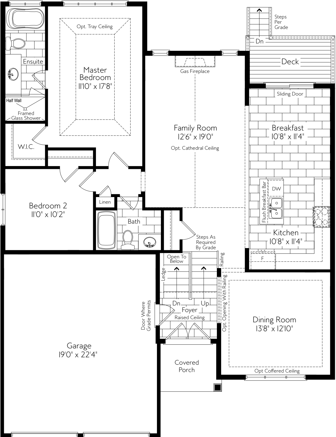
GROUND FLOOR ELEVATION A
