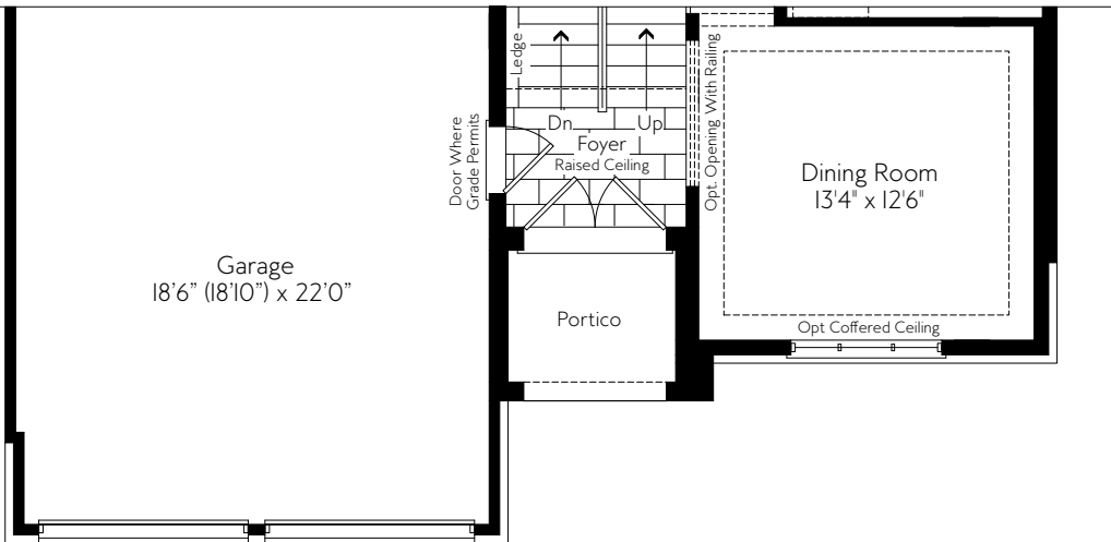
PARTIAL GROUND FLOOR ELEVATION B
