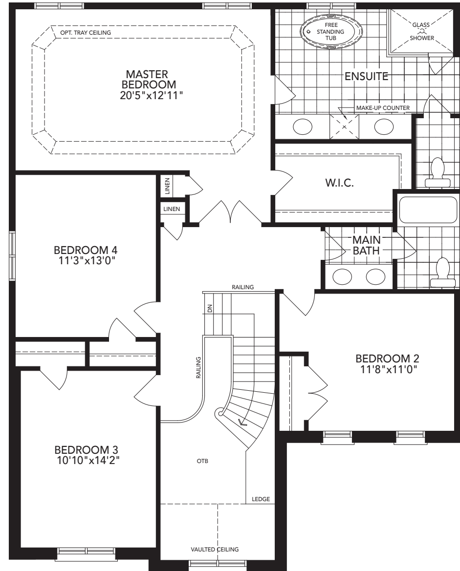
Second Floor - Elev. A
