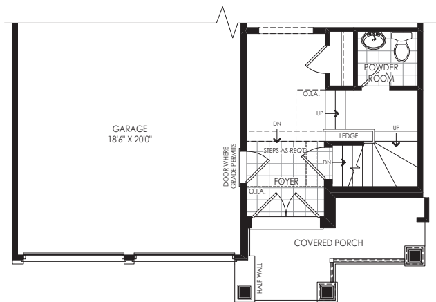
PARTIAL GROUND FLOOR EL. B
