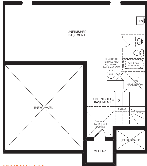
BASEMENT EL. A & B
