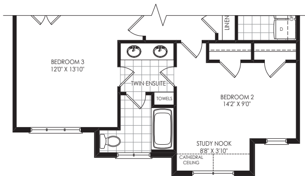
PARTIAL SECOND FLOOR EL. B
