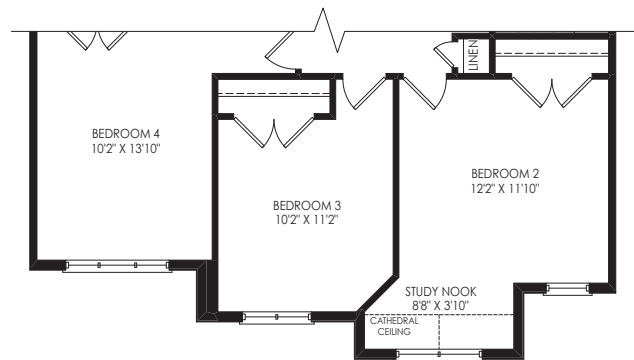
PARTIAL OPT. 4 BEDROOM SECOND FLOOR EL. B
