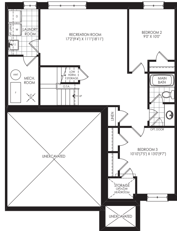
BASEMENT EL. A & B
