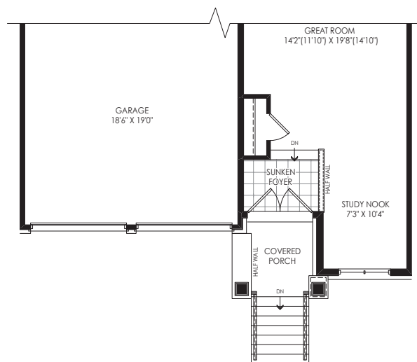
PARTIAL GROUND FLOOR EL. D RAISED CONDITION
