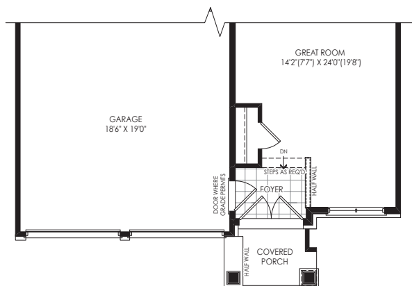
PARTIAL GROUND FLOOR EL. B
