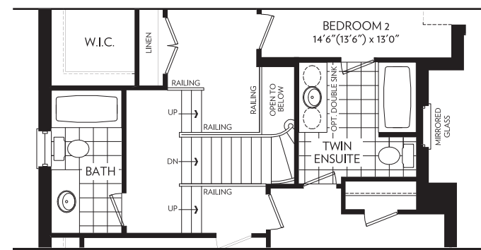
OPT. 3 BATHROOM SECOND FLOOR PARTIAL ELEVATION B
