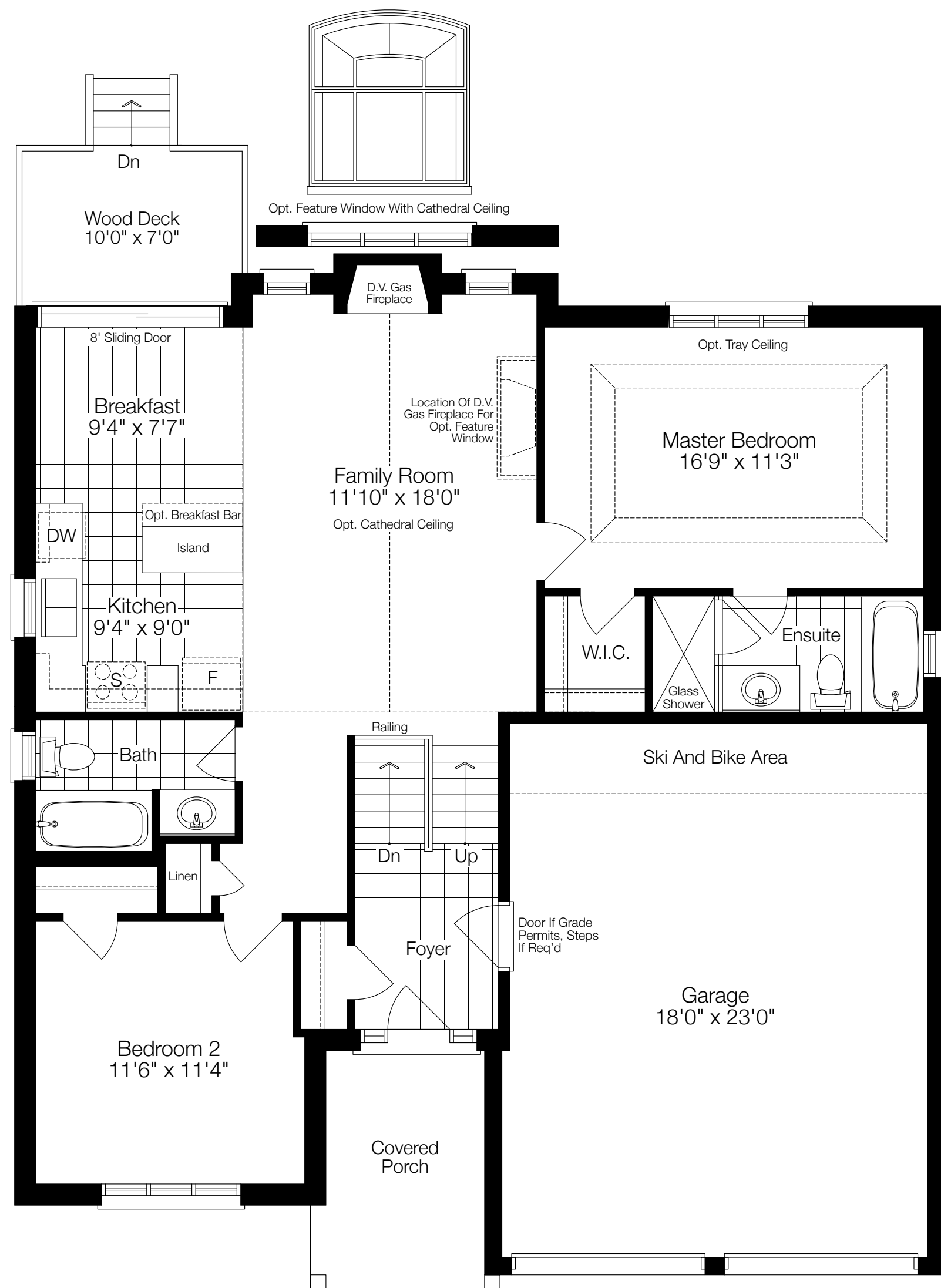
Ground Floor Elev. 'A'
