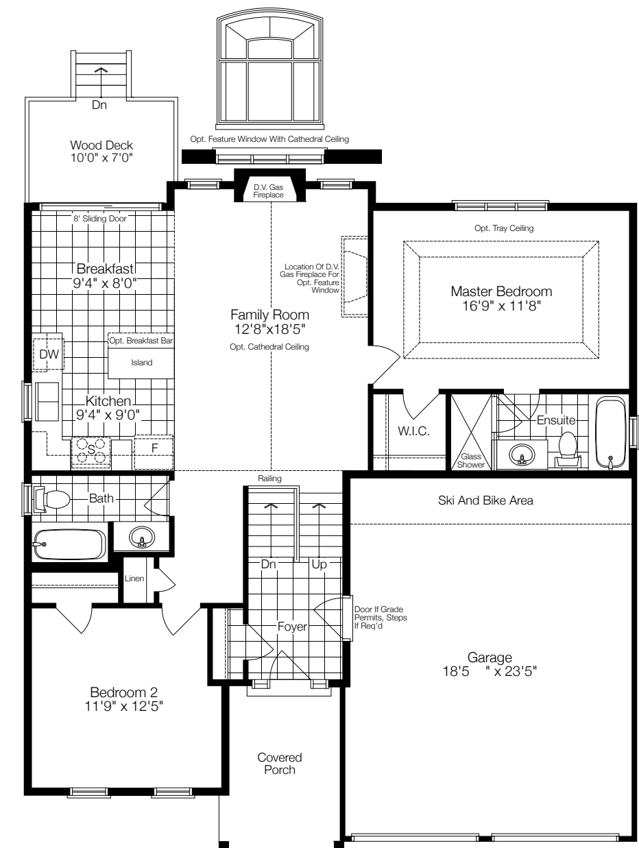
Ground Floor Elev. 'C'
