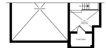
Partial Basement Elevation B
