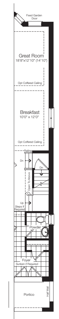
Partial Ground Floor End Condition Elev. A & B
