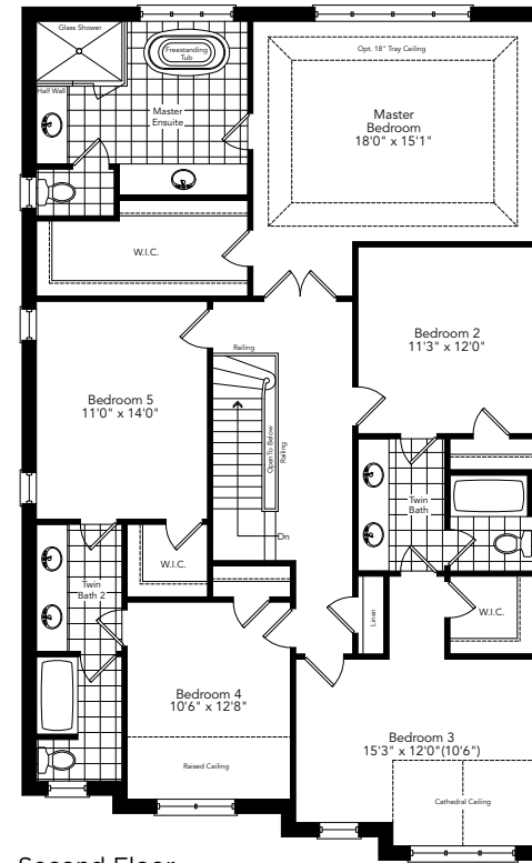
Second Floor Optional 5 Bedroom Plan Elevation A
