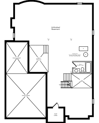
Basement Elevation A
