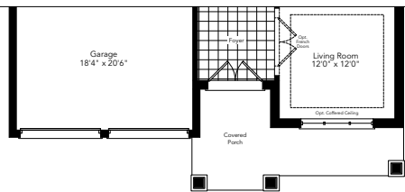
Partial Ground & Optional Ground Floor Elevation B
