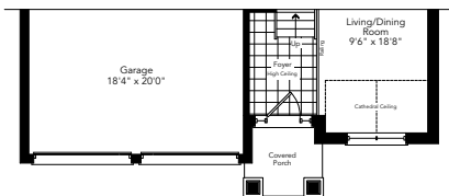
Partial Ground Floor Elevation B
