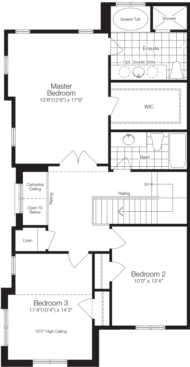
Second Floor Elev. B
