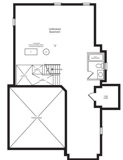
Basement Elevation B
