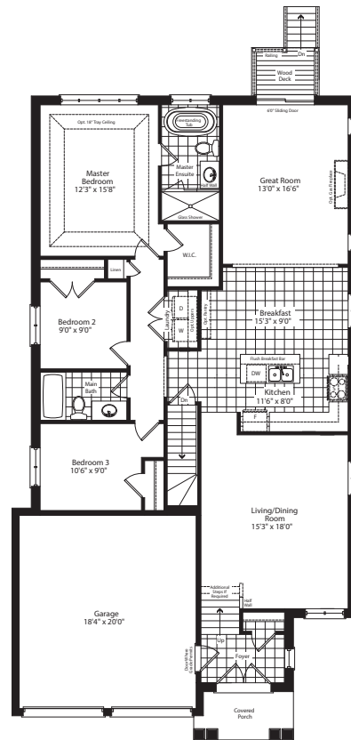
Ground Floor Optional 3 Bedroom Plan Elevation A
