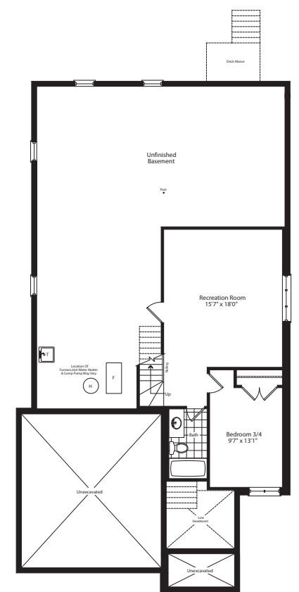
Optional Finished Basement Elevation A
