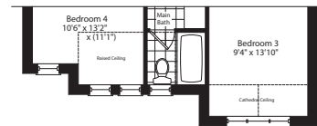
Second Floor Optional 4 Bedroom Plan Elevation A
